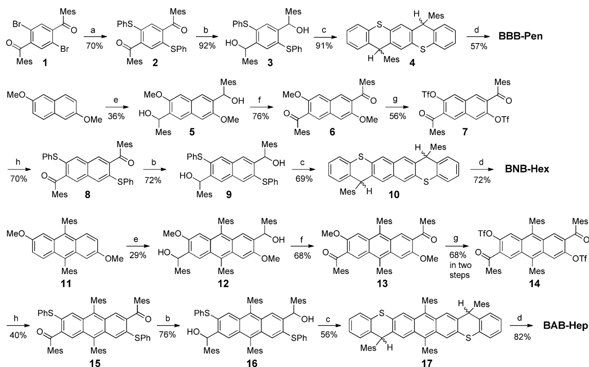
Scheme 1. Synthetic routes of BBB-Pen, BNB-Hex, and BAB-Hep: a) thiophenol, CuI, K 2 CO 3 , DMF; b) LiAlH 4 , THF; c) BF 3 ·Et 2 O, DCM; d) DDQ, toluene; e) i) n -BuLi, THF; ii) mesitaldehyde; f) PCC, DCM; g) i) BBr 3 , DCM; ii) Tf 2 O, pyridine, DCM; h) thiophenol, Pd 2 (dba) 3 , Xantphos, Cs 2 CO 3 . Mes = mesityl; DDQ = 2,3-dichloro-5,6-dicyano-1,4-benzoquinone; PCC = pyridinium chlorochromate, DCM = CH 2 Cl 2 .
